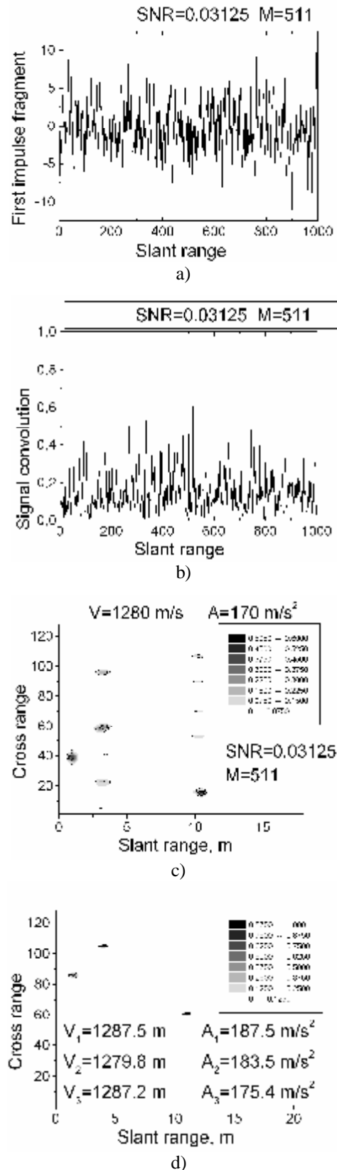
Fig. 2. Different stages of the signal processing: a) signal with noise at output of the phase discriminator; b) fragment of the compressed first impulse; c) the target image taking into account approximation parameters of target motion; d) final target image.
