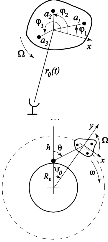
Fig. 1. The two-dimensional model of the target. Two model of the target motion.
